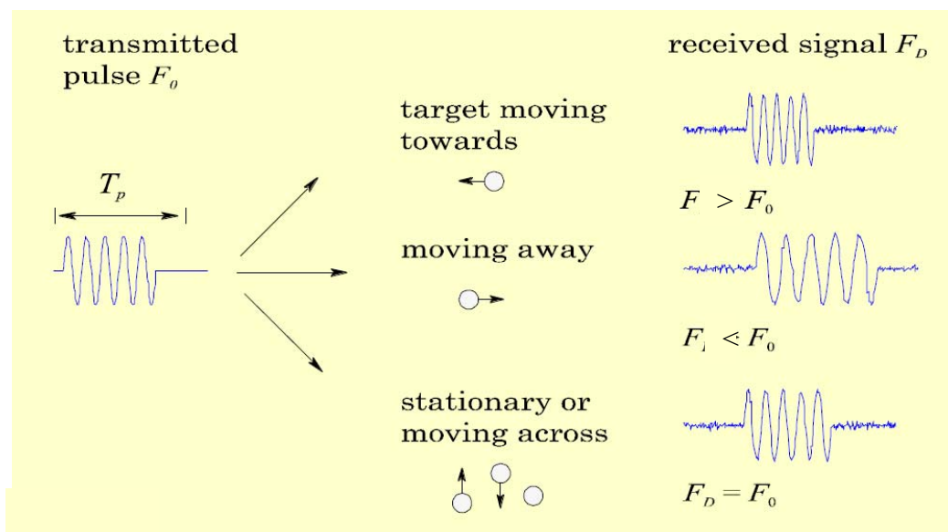
Figure 1. Measuring water velocity using a target with a monostatic Doppler system
