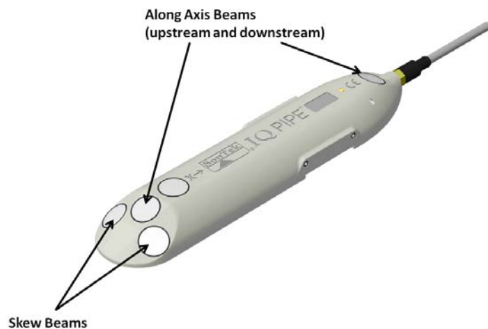
Figure 4. Beam geometry for the SonTek-IQ Pipe
