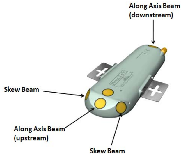
Figure 3. Beam geometry for the SonTek-IQ
